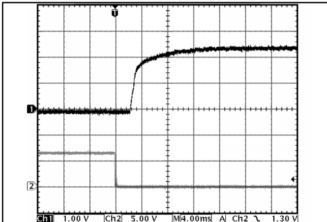
Figure 9: Turn-on transient at full load (resistive load) (4 ms/div). Input voltage pre-applied. Ch 1: V_{out} (1V/div), Ch 2: ON/OFF input (5V/div)
